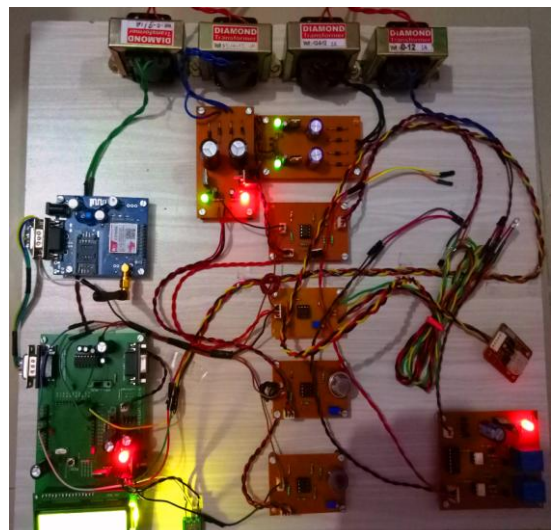
Fig.16.Photograph of fabricated project for GSM Operated Wireless Sensor Based Mine Security and Safety.
