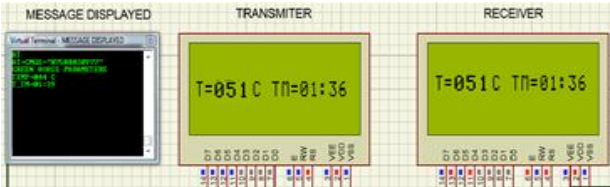
Fig. 5. Simulated results for temperature > 50°C.
