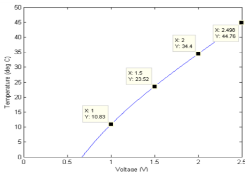
Fig. 6. Temperature sensor voltage relationship.
