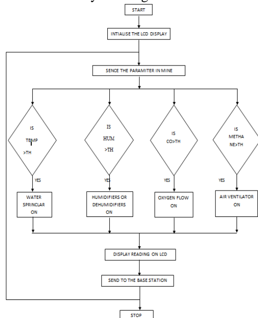
Fig. 3. flow chart for sensor section.
