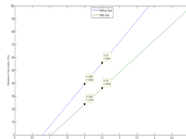
Fig. 9. Humidity sensor voltage relationship.
