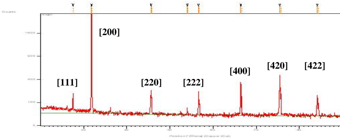
Figure 6. XRD of the natural salt extracted from the Ningel Thumkhong.
