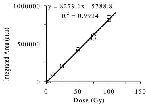
Figure 5. Dose response curve of the Salt extracted from Ningel Thumkhong.
