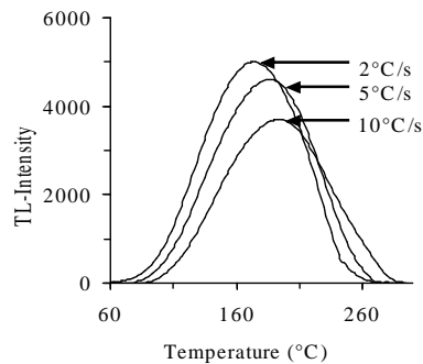
Figure 2. TL glow curves of the salt extracted from Ningel Thumkhong with different heating rates
