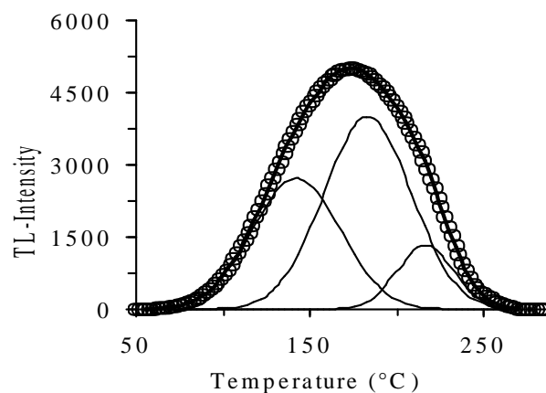
Figure 3. CGCD of salt extracted from Ningel Thumkhong for heating rate 2.0^\circ\text{C/s}^{-1} .
