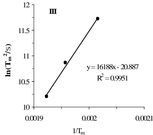
Figure 4. Plot of \ln(T_m^2/\beta) versus (1/T_m) .
