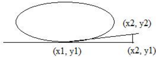
Figure 5: Computing angle
