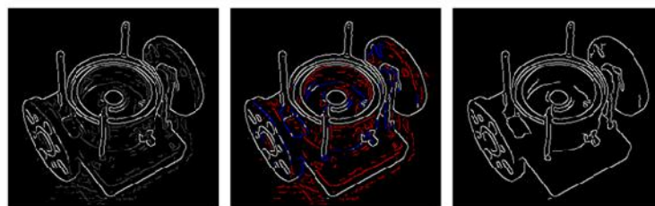
Figure 4: Blob Analysis
