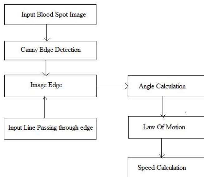
Figure 1: Proposed Model
