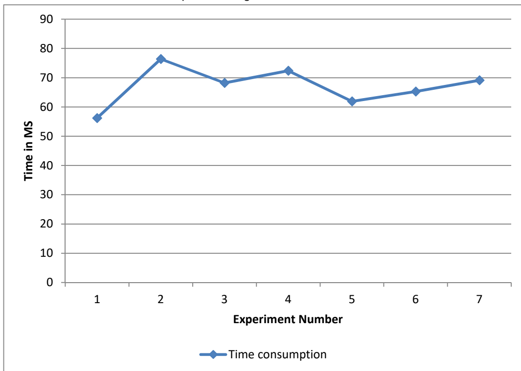
Figure 7: Time Consumption
