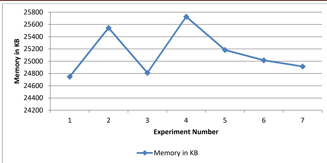
Figure 8: Memory Usages
