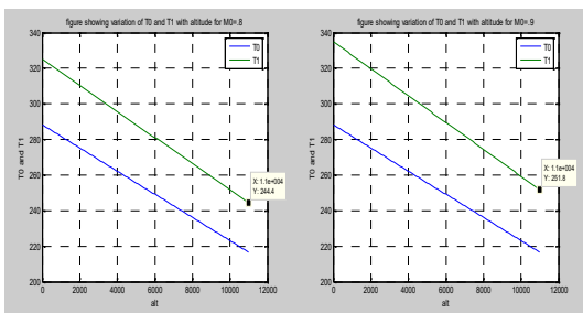
Figure4: showing variation of T_0 & T_1 with altitude for Mach number = 0.8 and 0.9.
